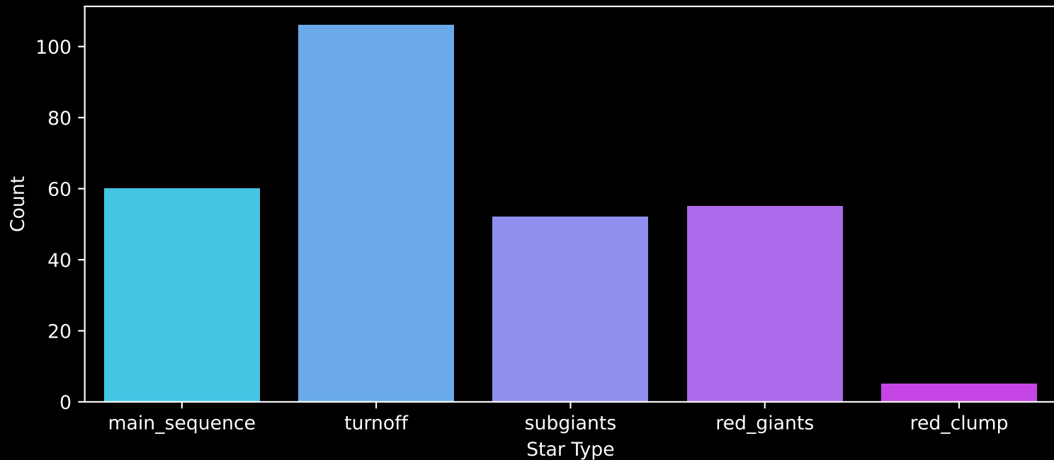
GALAH DR4 Field: [9275] Count plot of Star Type
