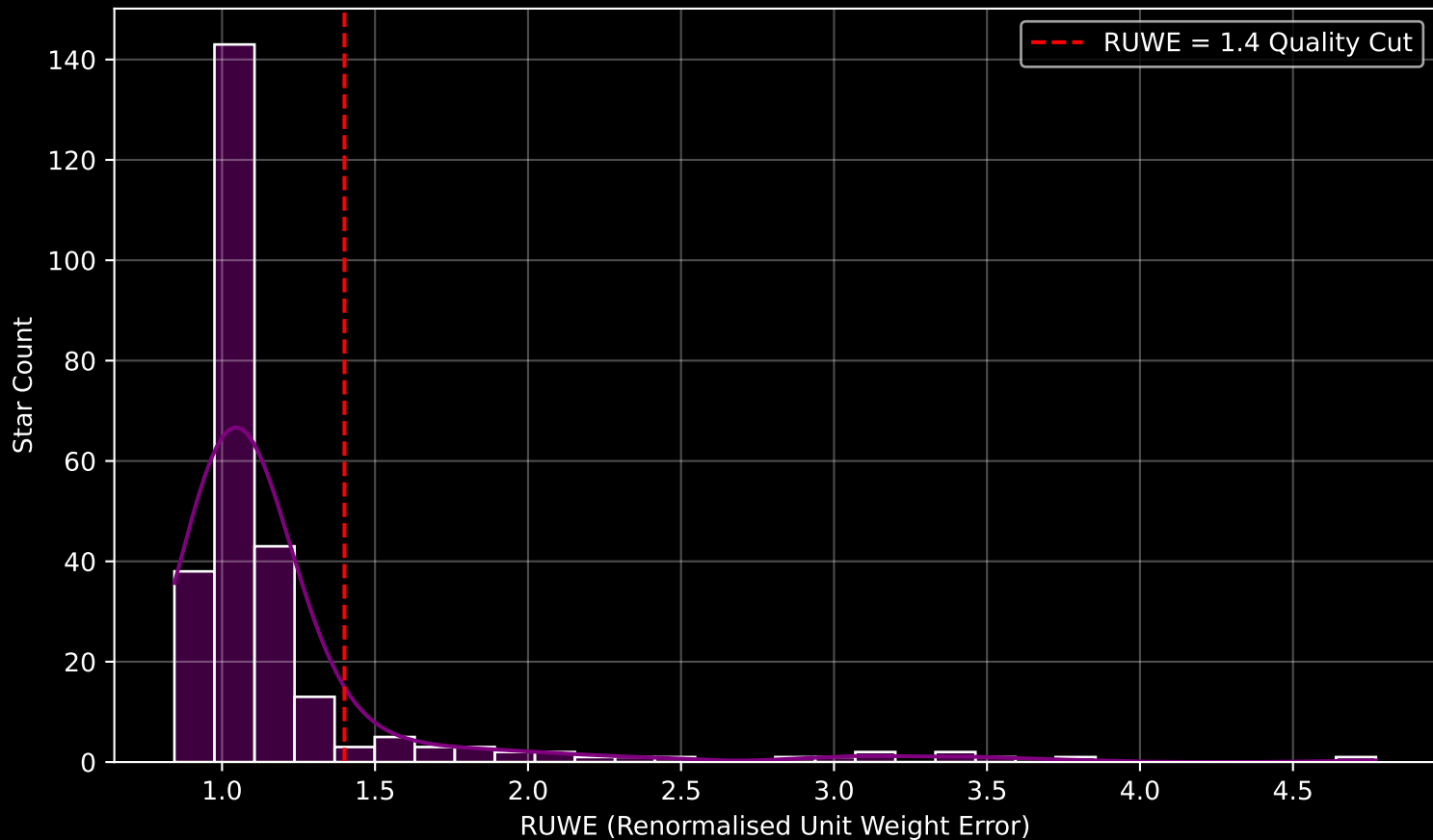
GALAH DR4 Field [9275] RUWE Distribution (n= 267)
