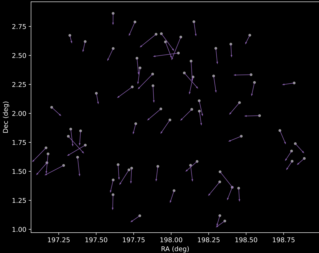
GALAH DR4 Cluster 8 Proper Motion Vectors (n=67)
